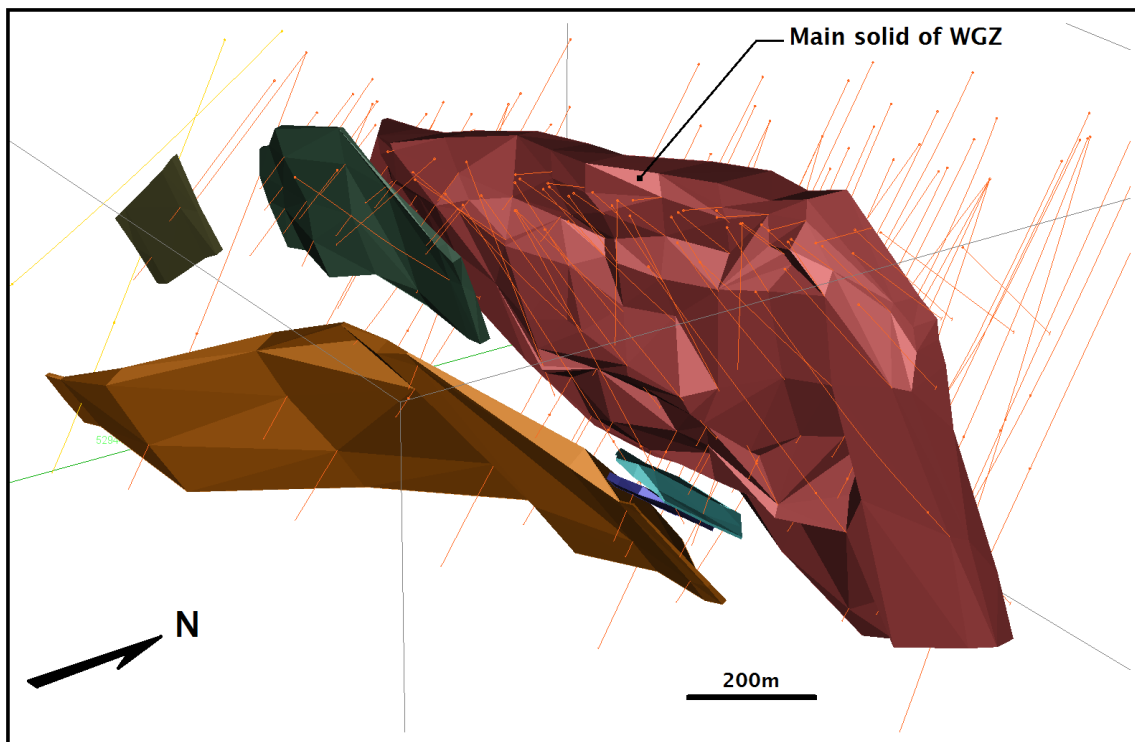
Figure 14.2 Elmtree 3D Isometric View of the Components of the WGZ and Diamond Drill Coverage
