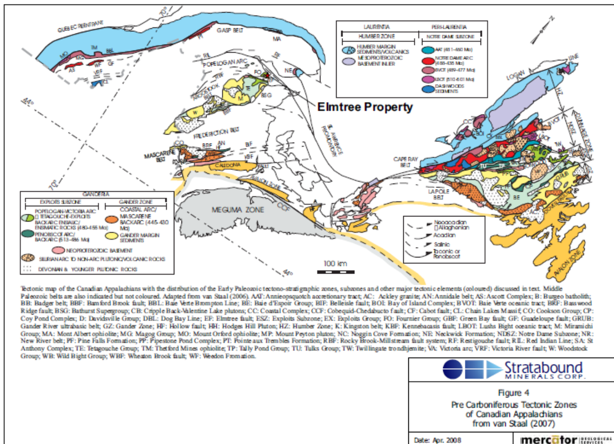
Figure 7.1 Regional Geology (1)
